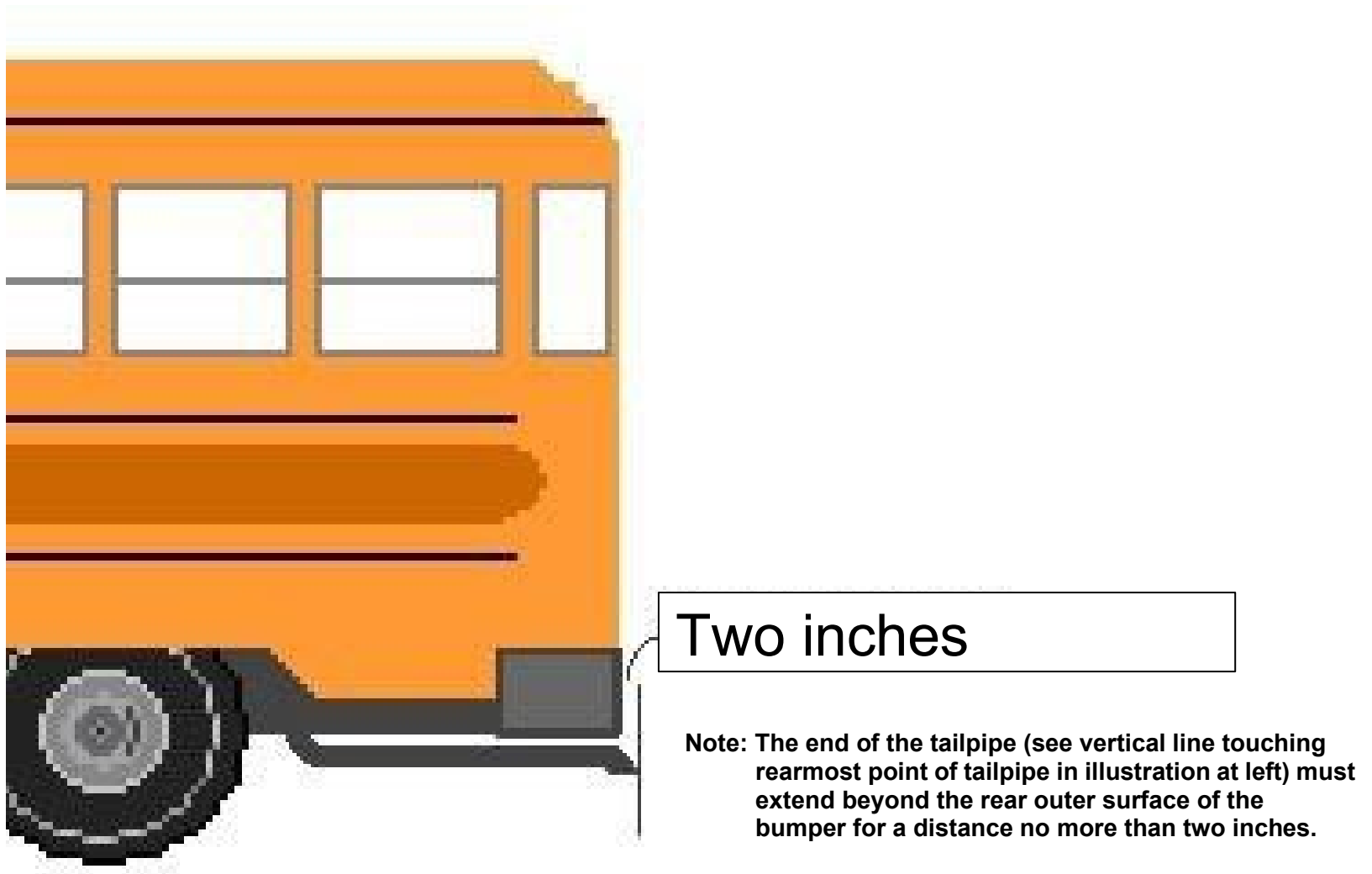
Figure 16 Tailpipe Length
